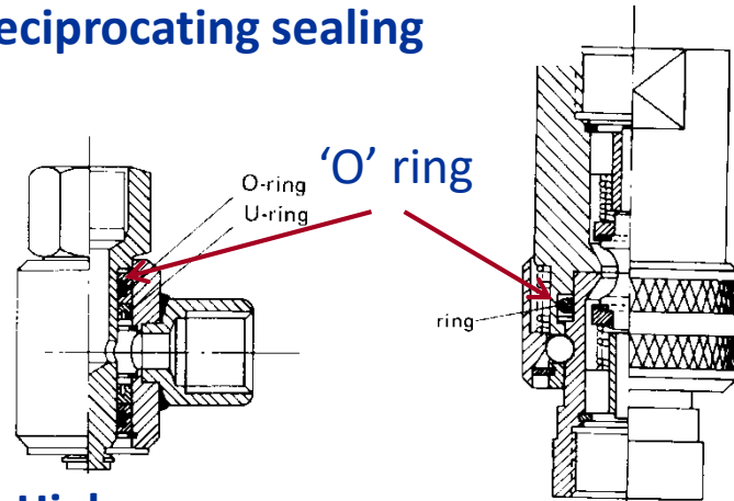
High pressure swivel coupling
