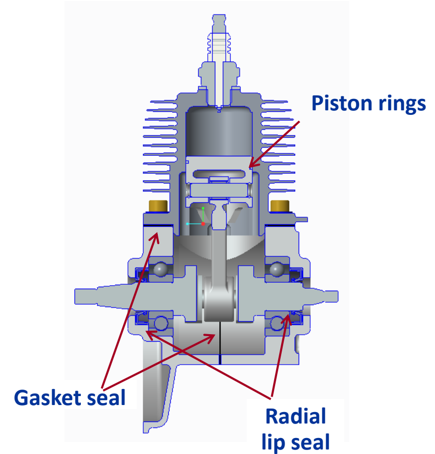
2-stroke engine
