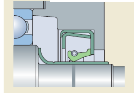
f) SKF radial lip seal with special wear sleeve
